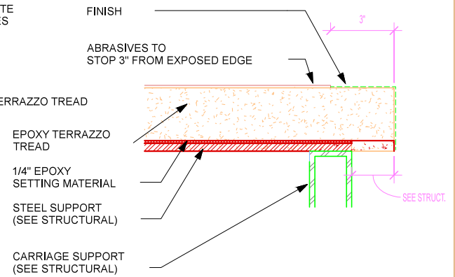
③ Tread Detail 3" = 1'-0"
