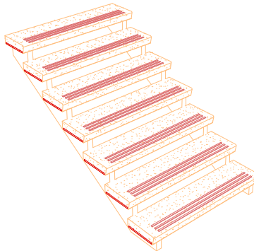
② PTE FS Carriage Tread - Tread Detail 1 3" = 1'-0"
