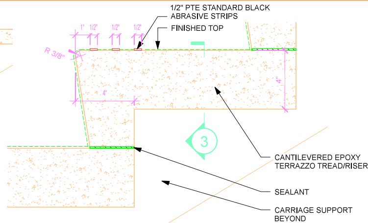
② Tread Detail 3" = 1'-0"
