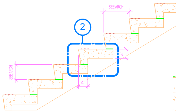
① Stair Section 3/4" = 1'-0"
