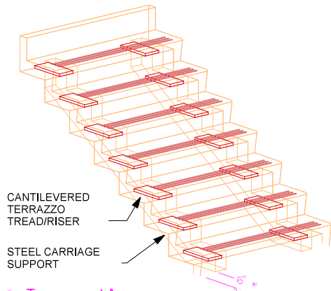
④ Transparent Axon
