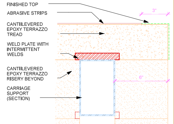
③ Tread Detail 3" = 1'-0"
