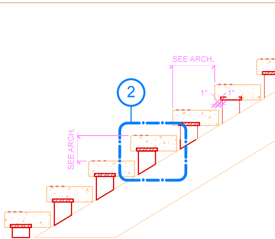
① Stair Section 3/4" = 1'-0"
