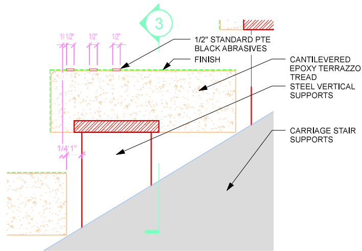
② Tread Detail 3" = 1'-0"
